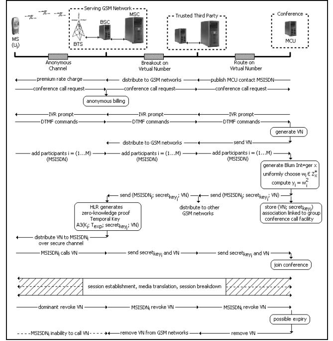
Fig. 3. Anonymous Invited Mobile Conference Call Facility Protocol
