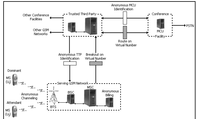
Fig. 1. Anonymous Mobile Conference Call Architecture
